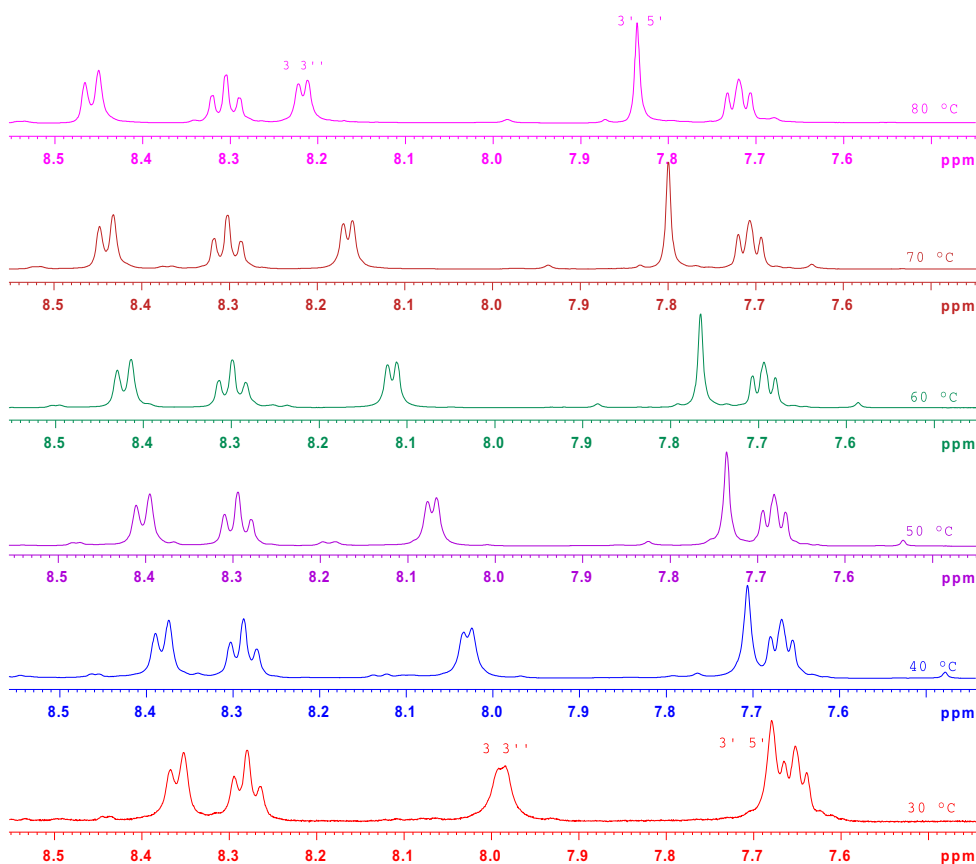
Figure 8. ^1\text{H} spectra of Ptdttteg (0.02 M) in DMSO- d_6 at 30–80 ^{\circ}\text{C} .
