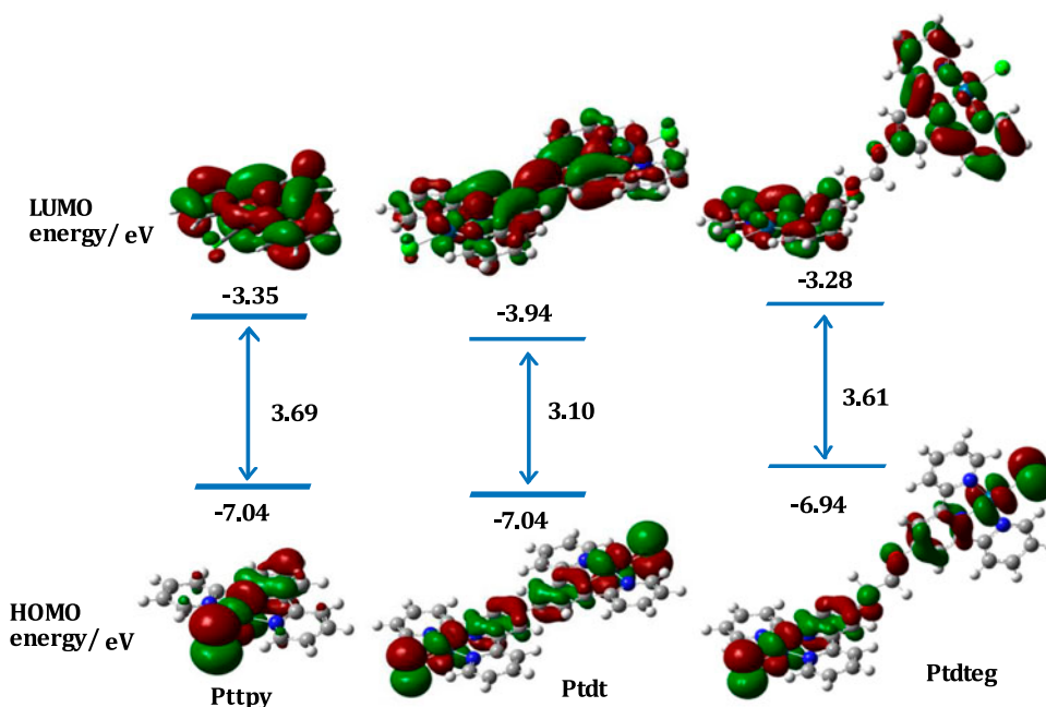
Figure 6. DFT-calculated minimum energy structures, frontier molecular orbitals (HOMO and LUMO) of Pttpy, Ptdt, and Ptdteg. Data for Pttpy are included for comparisons. Data for Ptdtdeg, Ptdtgeg, and Ptdttgeg are included in figure S1 (Supporting Information).
