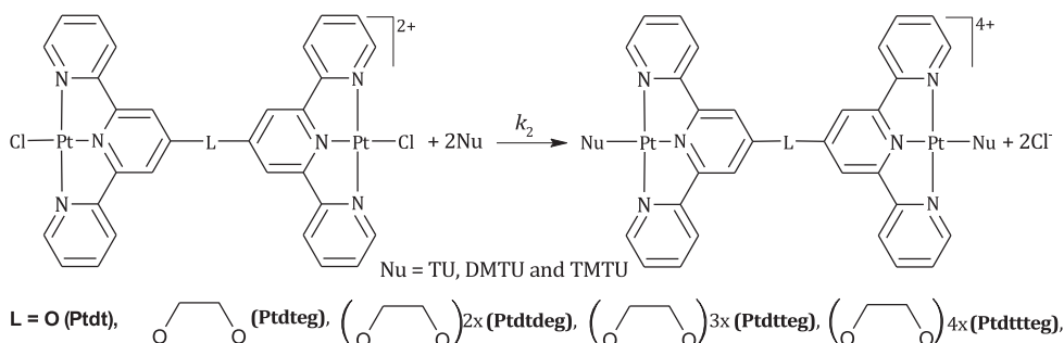
Scheme 1. Proposed substitution mechanism for the dinuclear Pt(II) complex system with thiourea nucleophiles.
