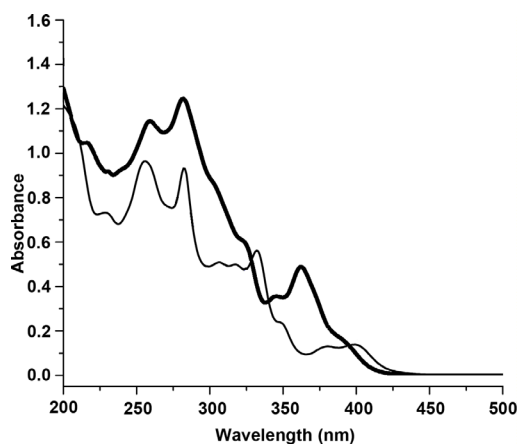
Fig. 2. Absorption spectra measured in acetonitrile for [\text{Pt}\{4'\text{-(}o\text{-tolyl)trpy}\}\text{Cl}]^+ (thin line) and [\text{Pt}\{4\text{-(}o\text{-tolyl)isqbipy}\}\text{Cl}]^+ (thick line).
