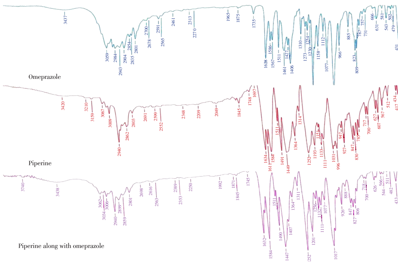
Figure 1. FTIR details of pure omeprazole and piperine with important IR bands.
