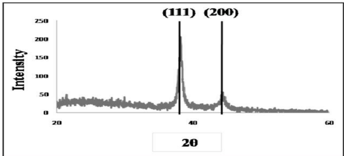
Figure 3. XRD pattern of the silver nanostructures grown on ITO.
