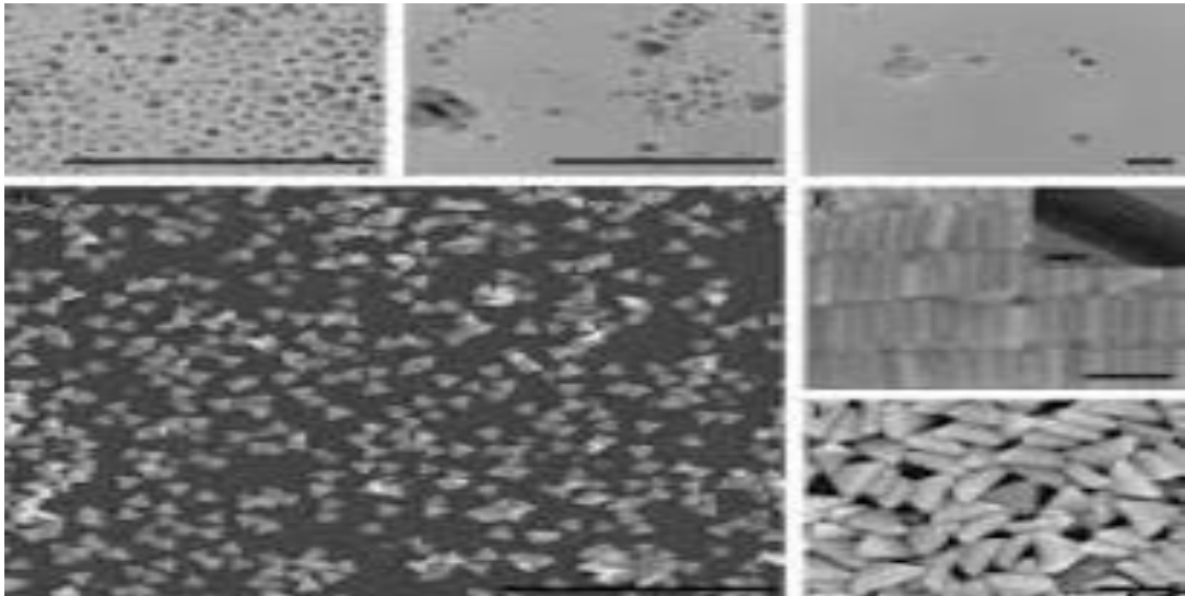
Figure 2: Lattice pattern of the silver nanoparticle on the surface of Indium tin oxide
